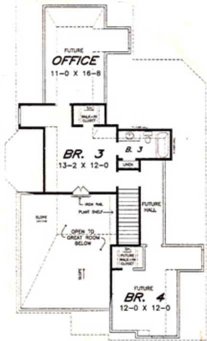
Second Floor Plan (A)
