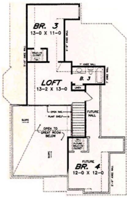
Copyright 2002 Ralph Jones Second Floor Plan
